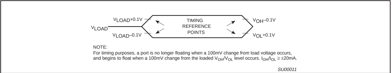
Figure 51. Float Waveform
